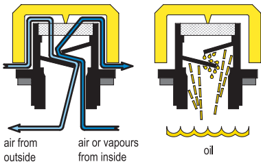
Operating layout
