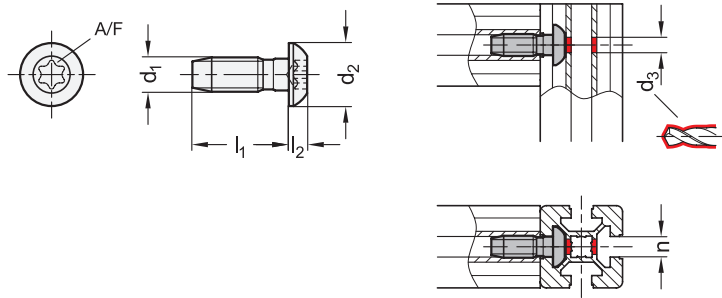
Assembly / profile machining
